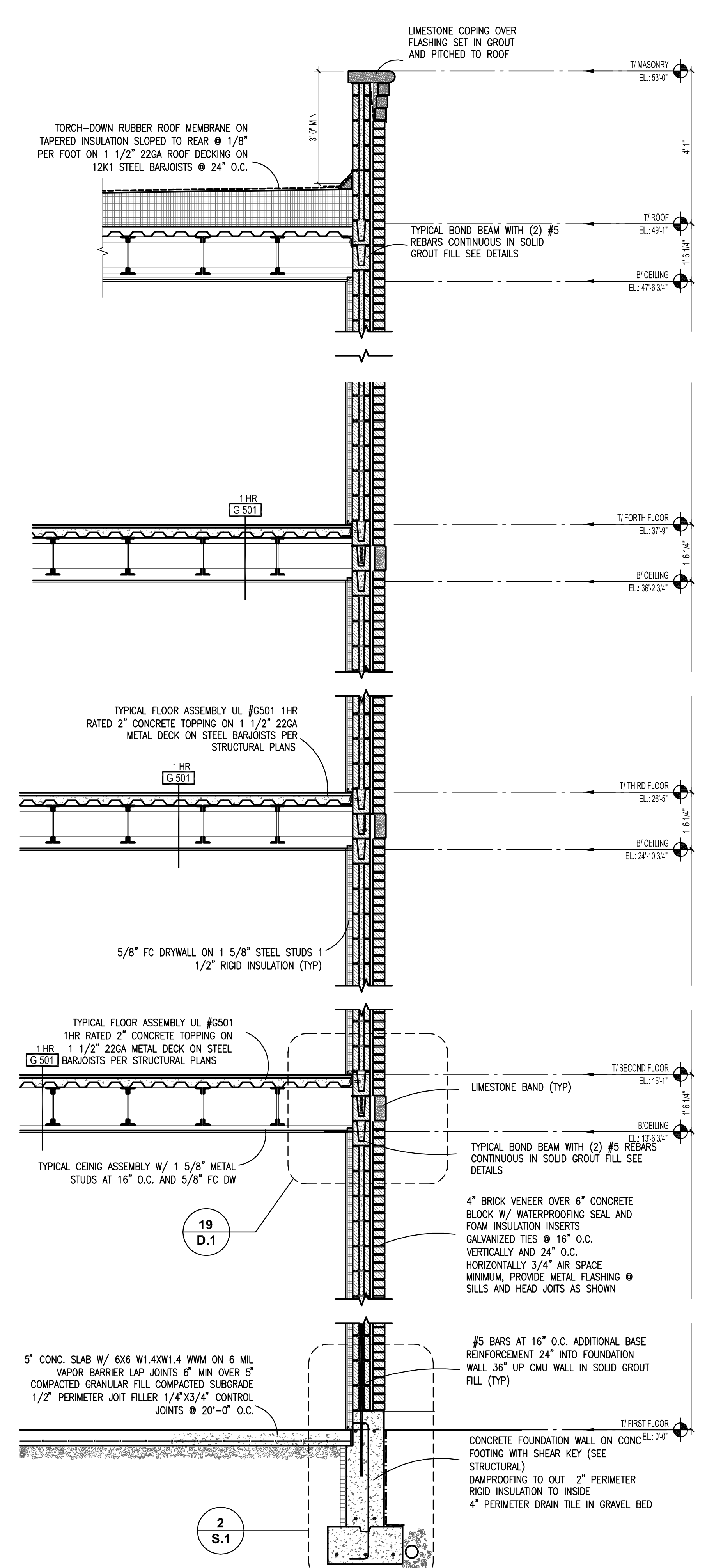
SECTION A.6 SCALE: 1/2" = 1'-0" 0 2' 4'
