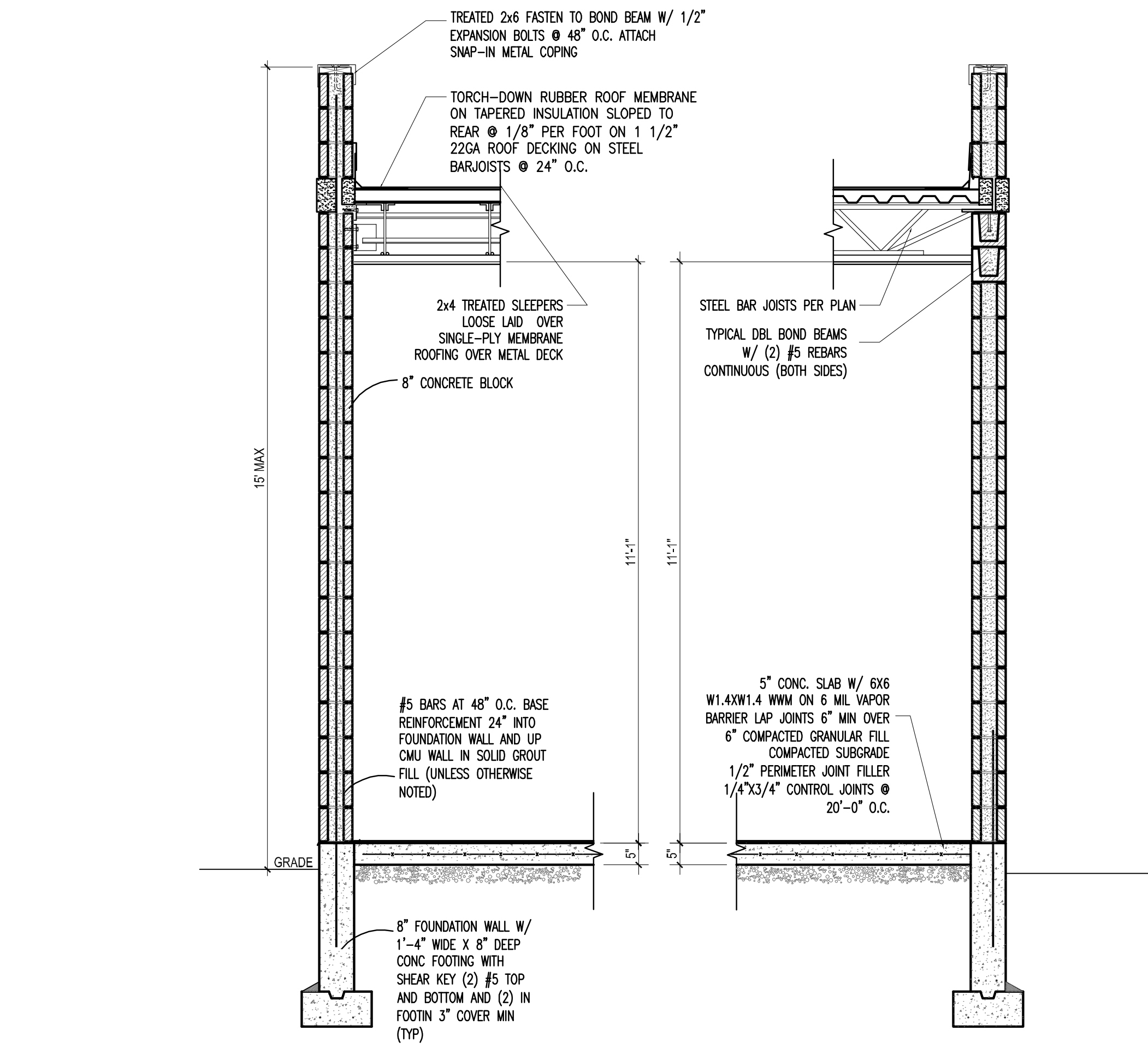
SECTION A.6 SCALE: 1/2" = 1'-0" 0 2' 4'
