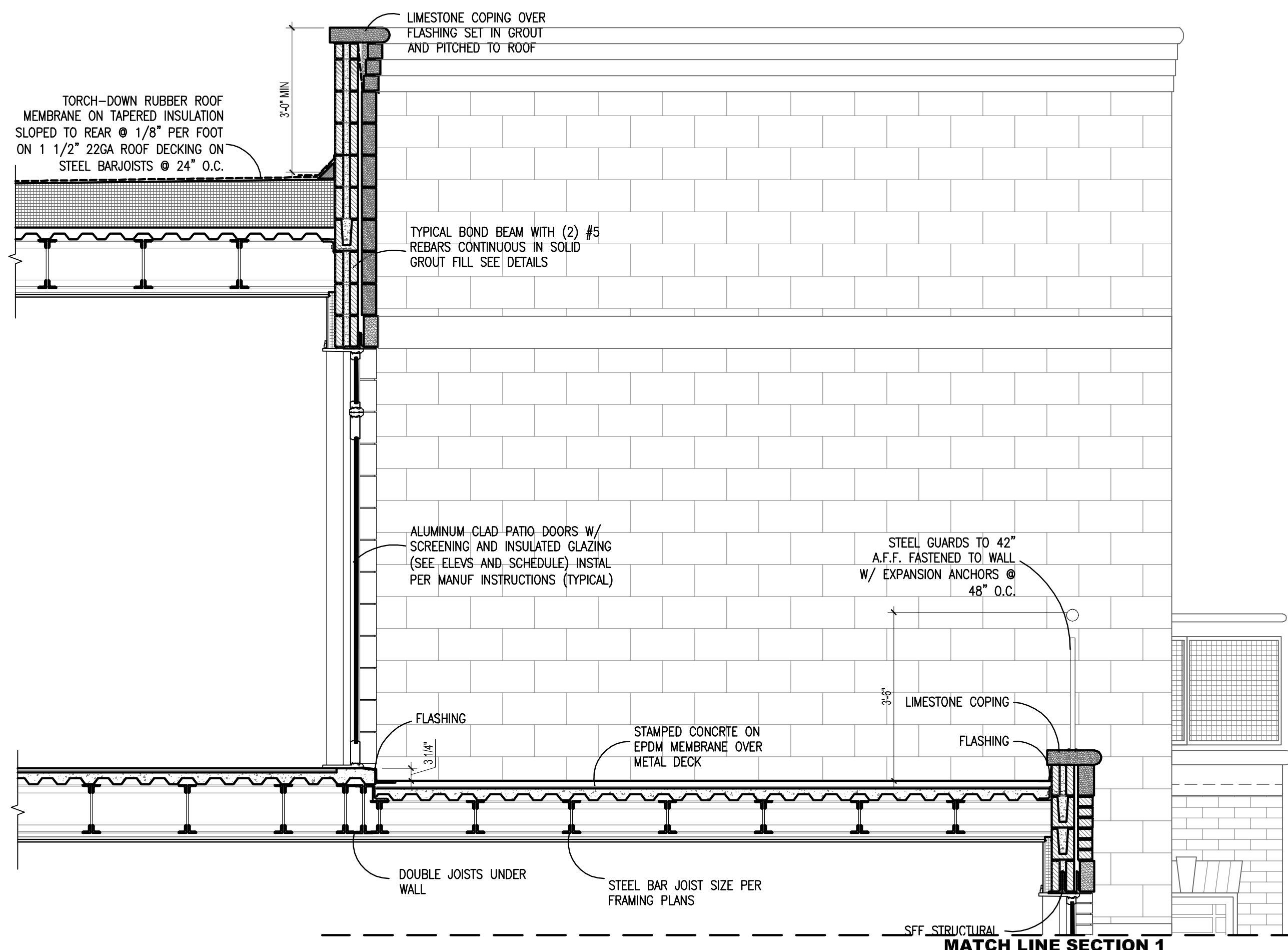
SECTION A.6 SCALE: 1/2" = 1'-0" 0 2' 4'
