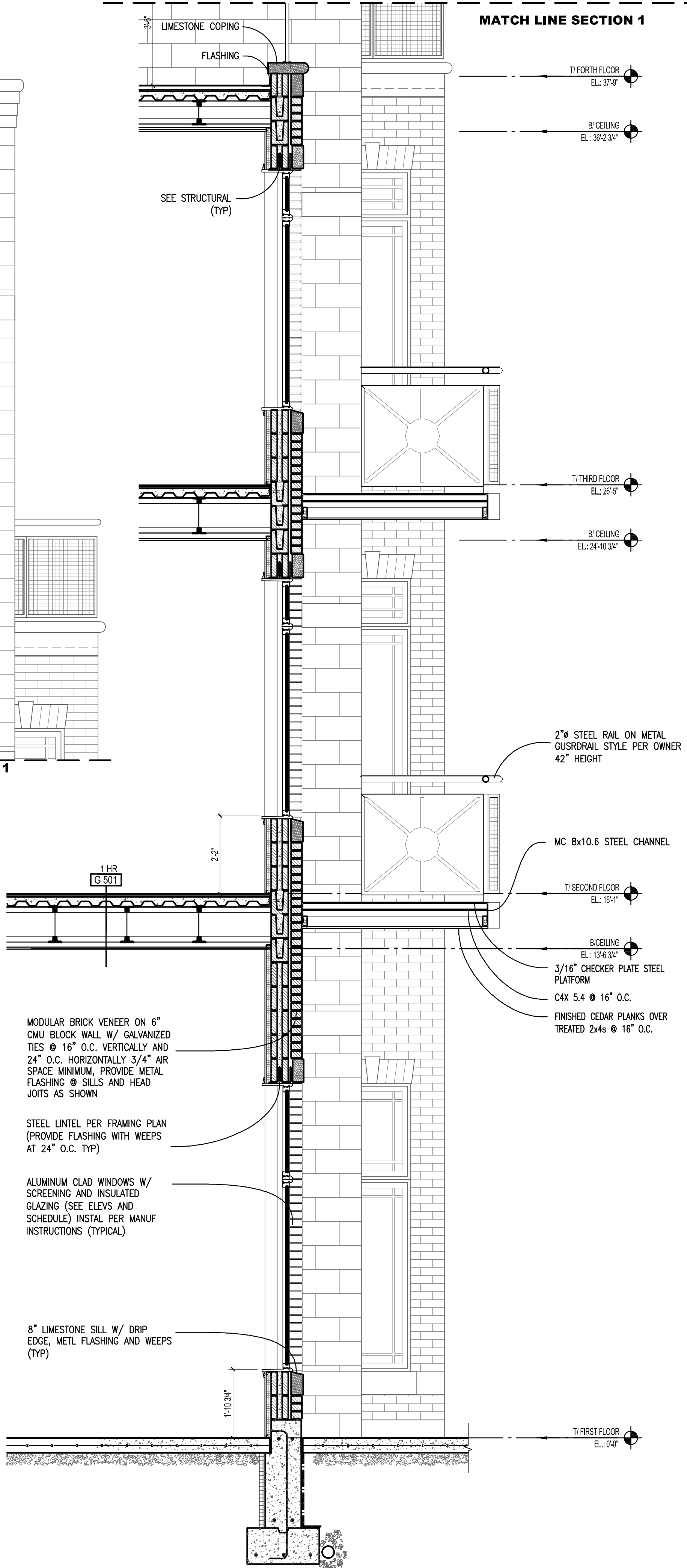
SECTION A.6 SCALE: 1/2" = 1'-0" 0 2' 4'
